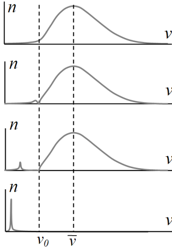
Figure 2. The evolution of the time velocity distribution during the cooling of the slow part of the atoms in the Zeeman slower. The lowest graph corresponds to the moment when the fast atoms have left the slower.
