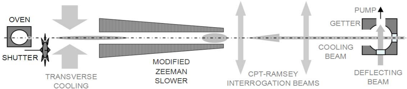
Figure 1. Scheme of the atomic beam preparation/registration unit of the satellite clock.
